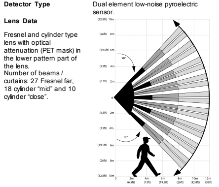
Figure 12 – Coverage Pattern Walk Test
